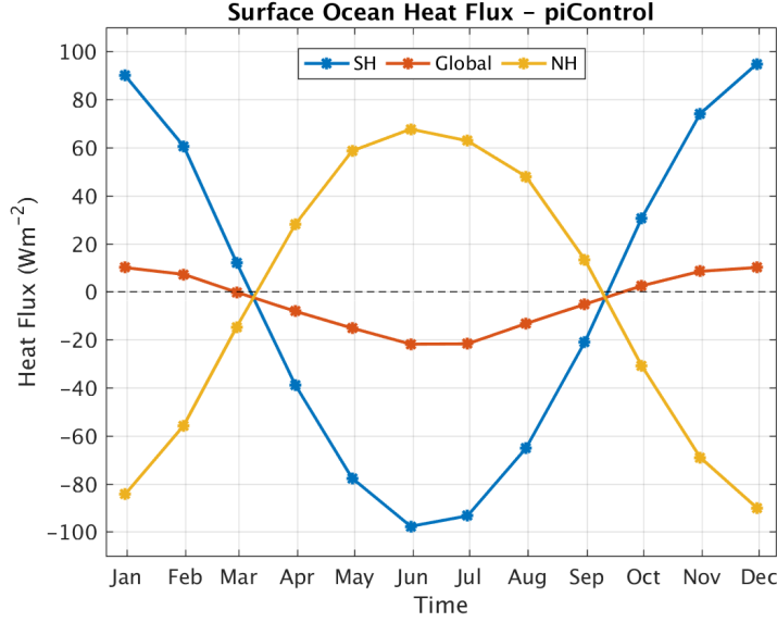
Figure 48: Average annual cycle of the surface heat flux for the entire globe, and separated by hemisphere. SH denotes Southern Hemisphere, and NH denotes Northern Hemisphere. The black dashed line marks the zero.
