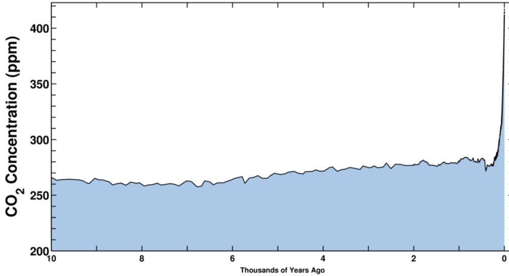
Figure 8: Historical time series of CO 2 concentration over the last 10,000 years from ice-core data, before 1958, and from Mauna Loa observations, post 1958. Source: Taken and modified from The Keeling curve website ( https://scripps.ucsd.edu/programs/keelingcurve/ ).
