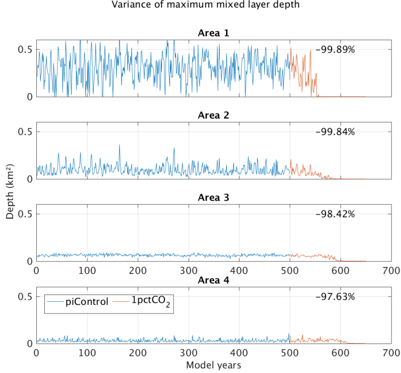
Figure 64: Variance time series (in \text{km}^2 ) for the mixed layer depth of Figure 63. The texts inside the time series represent the reduction in the variability in the last decade of the 1pctCO 2 experiment.
