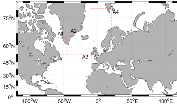
Figure 44: Locations of the four areas chosen to monitor the mixed layer depth time series.
