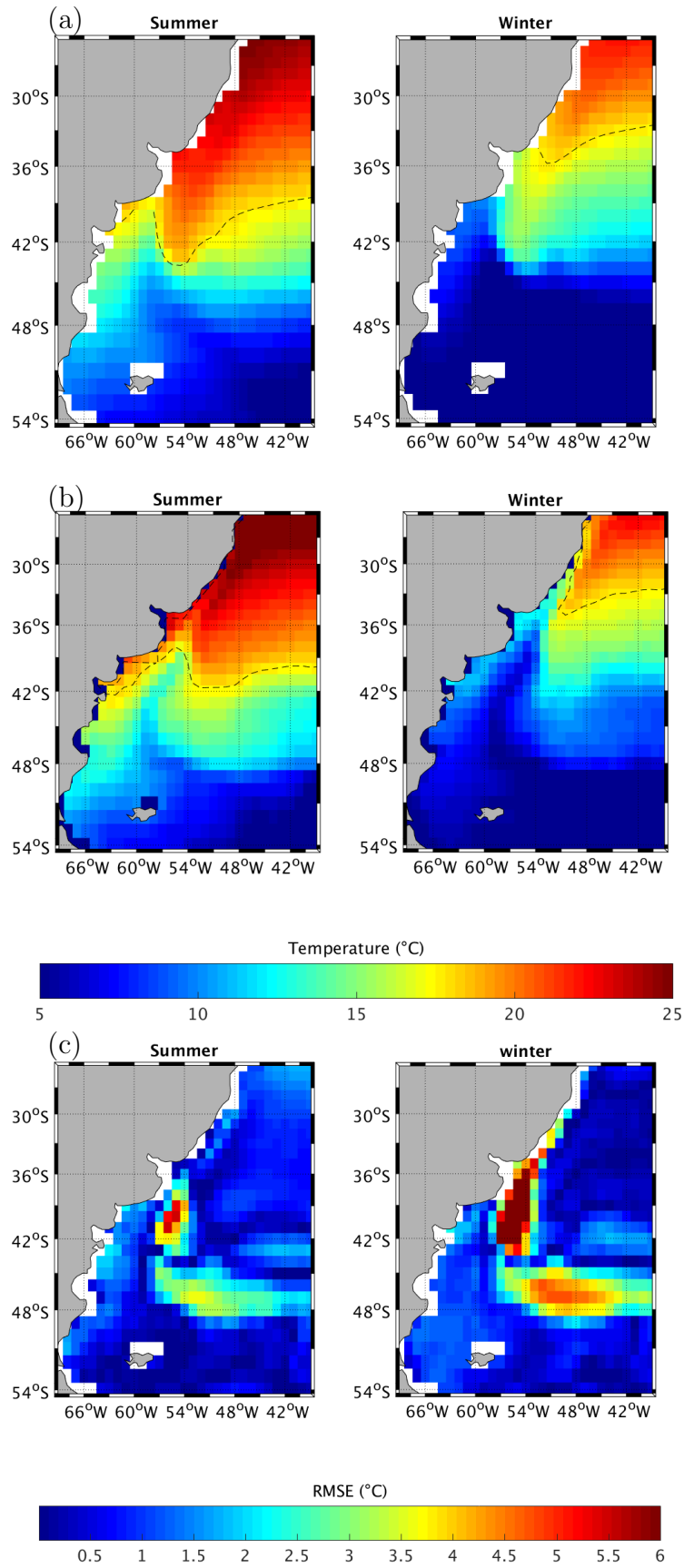
Figure 52: Seasonality of the Brazil-Malvinas Confluence in summer and winter for the (a) average of piControl and (b) average of CMEMS product. The black dashed line represents the 18°C isoline delimitation. Additionally, (c) depicts the RMSE between them.
