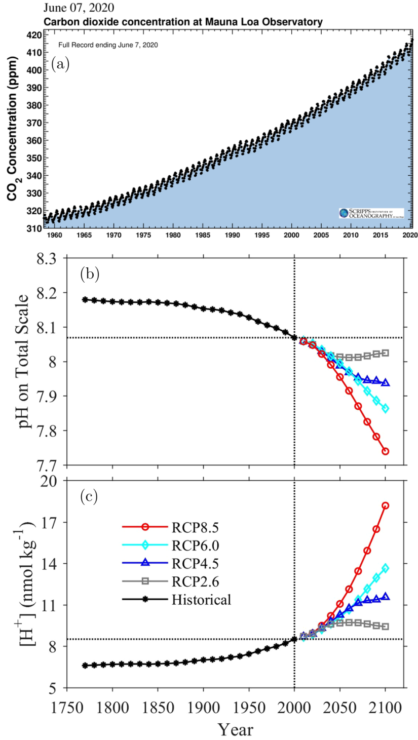
Figure 3: (a) Atmospheric concentrations of CO 2 since 1958 from Mauna Loa Observatory in Hawaii (19.5°N and 155.6°W) and time-series for (b) pH and (c) H + for historical and RCPs projections. Source for (a): Taken and modified from The Keeling curve website ( https://scripps.ucsd.edu/programs/keelingcurve/ ). Dataset is available at KEELING and KEELING, 2017 . Source for (b) and (c): Modified from JIANG et al. , 2019 .
