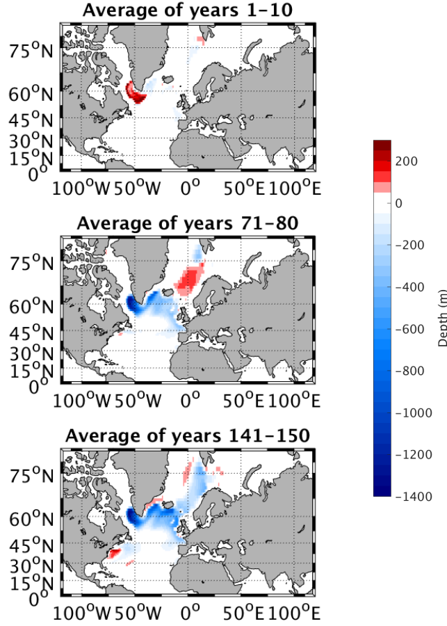
Figure 62: Mixed layer depth anomaly in March for average years 1-10, 71-80, and 141-150 compared to the average of the piControl experiment. Positive (negative) values indicate an increase (decrease) in the mixed layer depth.
