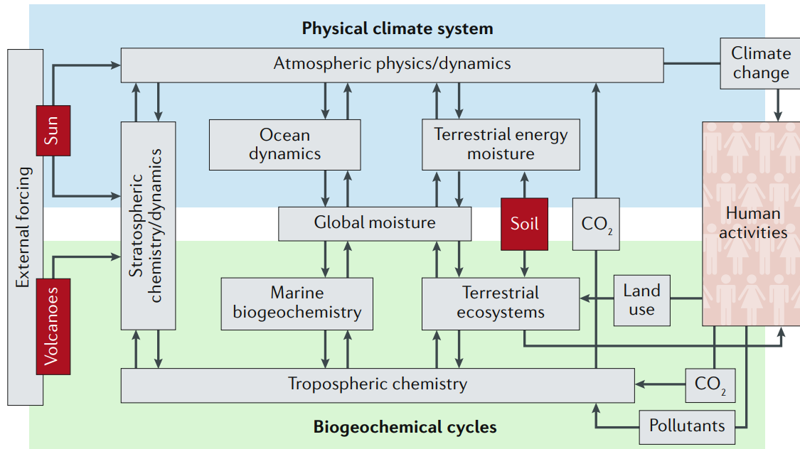
Figure 5: Scheme representing the Earth System and its interactions. Source: STEF-FEN et al., 2020 .
