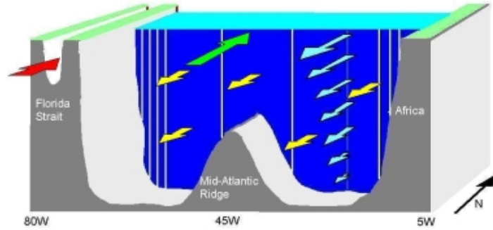
Figure 24: Scheme of MOC transport through the 26.5^\circ\text{N} parallel. The red arrow represents the Florida Strait transport, the green one the Ekman transport, the blue arrows are related to the induced density transport, and the yellow arrows represent the correction made to the velocity. Source: RAPID, 2019 .
