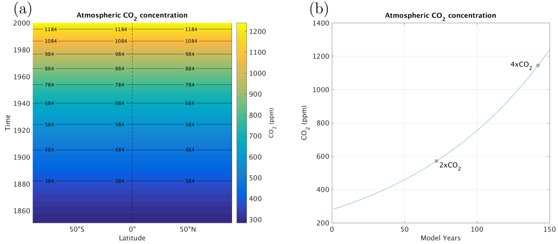
Figure 39: Atmospheric \text{CO}_2 concentration forcing (a) over latitude and (b) on average. The two points on the curve in (b) identify where the \text{CO}_2 concentration doubles and quadruples.
