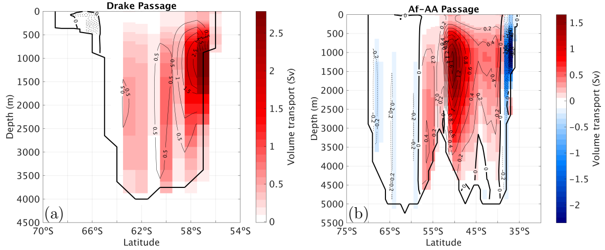
Figure 49: Volume transport profile for the average of piControl across (a) the Drake Passage and (b) Africa-Antarctic Passage. The colors depict the intensity and direction of the flow; red means eastward flow, and blue means westward flow. Additionally, contours show the transport values in Sv; continuous lines for eastward flows and dashed ones for westward flows.
